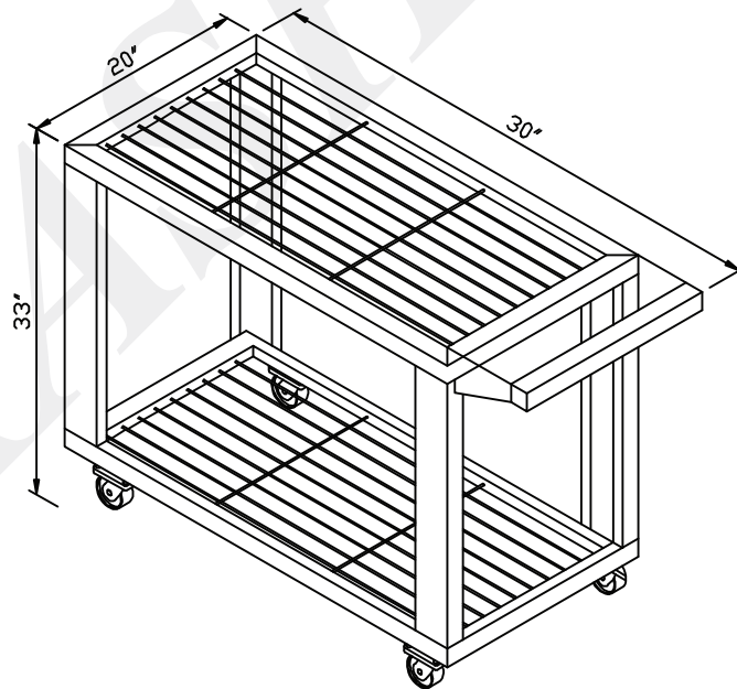
L) MULTIPURPOSE ROD SHELVES TROLLEY
