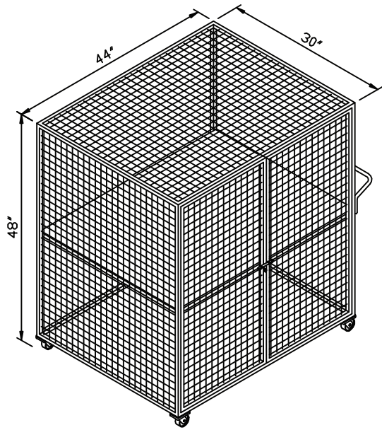
J) SHIPPER TROLLEY (CLOSED TYPE)
