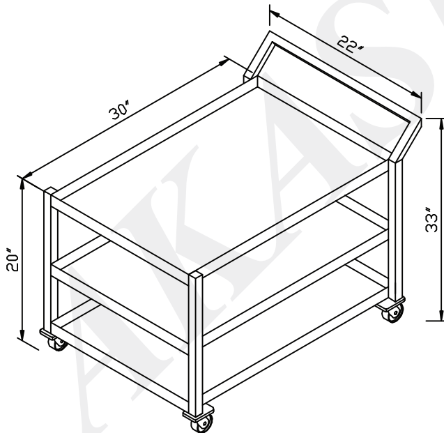
E) MULTIPURPOSE TROLLEY-3 TIER
