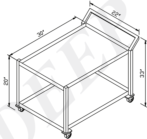
D) MULTIPURPOSE TROLLEY - 2 TIER
