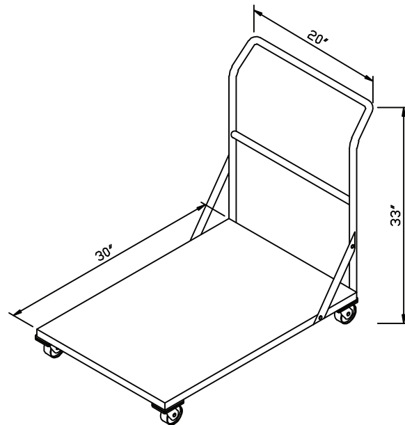
F) PLATFORM TROLLEY
