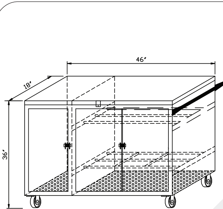
(C) SIEVES TROLLEY WITH SIDE CABINET
